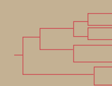
Tree Diagram
